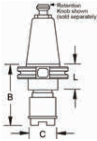
CAT50 Shank
