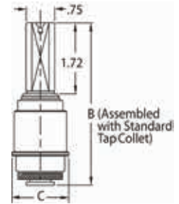
Straight Shank
